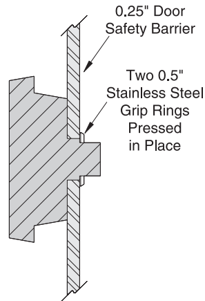
Section of Mounted Knob
