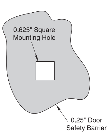
Mounting Provision for Elliott Barrier Knob (Square Mounting Provision Prevents Rotation of the Barrier Knob)
