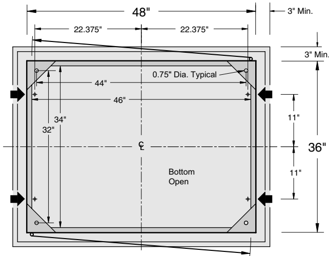
Section BB with Typical Pad Dimensions
